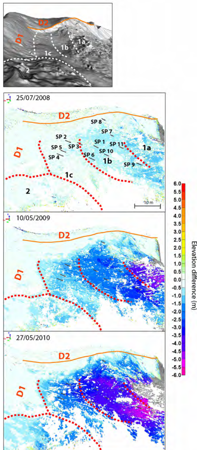
Fig. 10 TLS point cloud comparisons according to the reference date of 18 May 2008. The displacements are calculated with the shortest distance comparison in the vertical direction. A negative value means that the point elevation is lower than the point of the reference. Several blocks are clearly individualized through time. The blocks 1a, 1b and 1c belong to the sub-unit 1. The block 2 belongs to the sub-unit 2. The displacement vectors of the SPs are also indicated.
