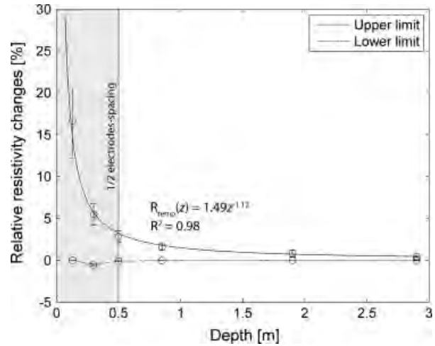
Figure 4. Maximum of relative resistivity variation caused by soil temperature changes. The maximum of relative resistivity changes are located above 0.5 m depth. Above that depth, the inverted resistivity models are poorly resolved (less than 0.5 electrode spacing)
