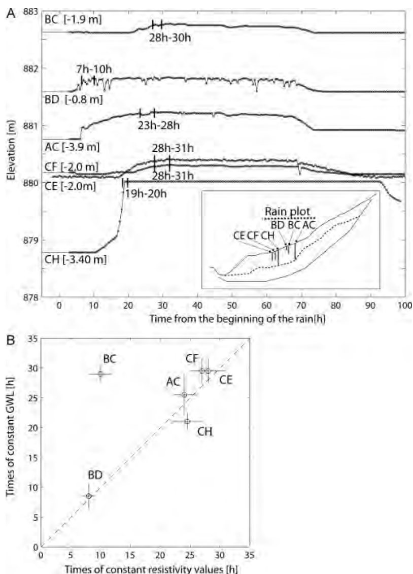
Figure 9. (A) Ground water level changes in piezometers located along the ERT line. After a certain time the groundwater level remains constant until the end of the rain experiment. [ \times m] is the piezometer depth. (B) Comparison with the time of constant resistivity values with the time of constant ground water level observed in the piezometers
