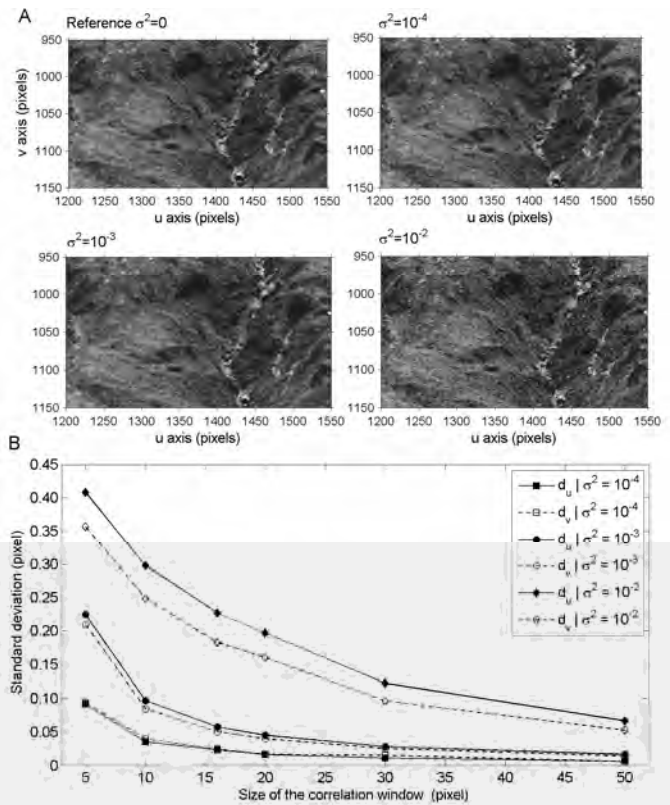
Fig. 10. Precision of the correlation algorithm. (A) Examples of different level of Gaussian noise introduced in the images; (B) Precision of the hierarchical correlator in the u and v direction as a function of different levels of Gaussian noise ( \sigma_n^2 ) and different sizes of the correlation window
