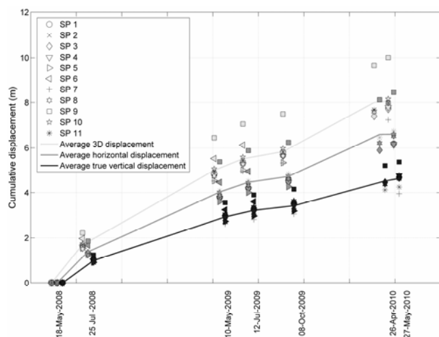
Fig. 11 Cumulated displacements of the SPs calculated with the rotation-translation technique.
