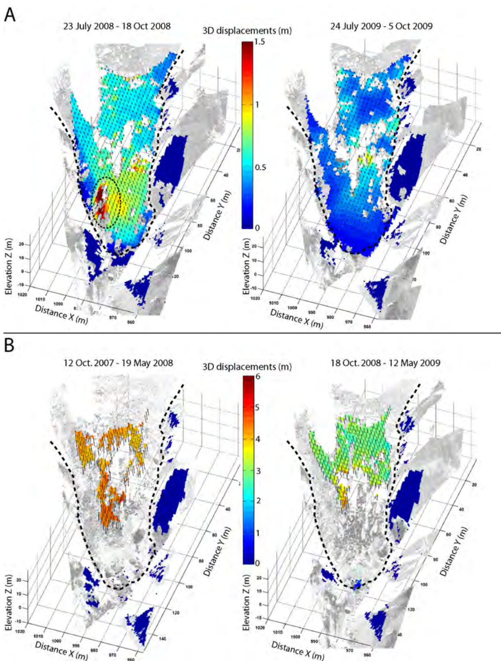
Fig. 9. 3D displacements field obtained by TLS measurements related to the acquisition periods of (A) July - October of the years 2008 and 2009, and (B) the periods of October - May of the years 2007 and 2008. The dashed circle indicates the detachment of some material at the front of the toe. The displacement maps are draped on their corresponding point clouds (intensity values).
