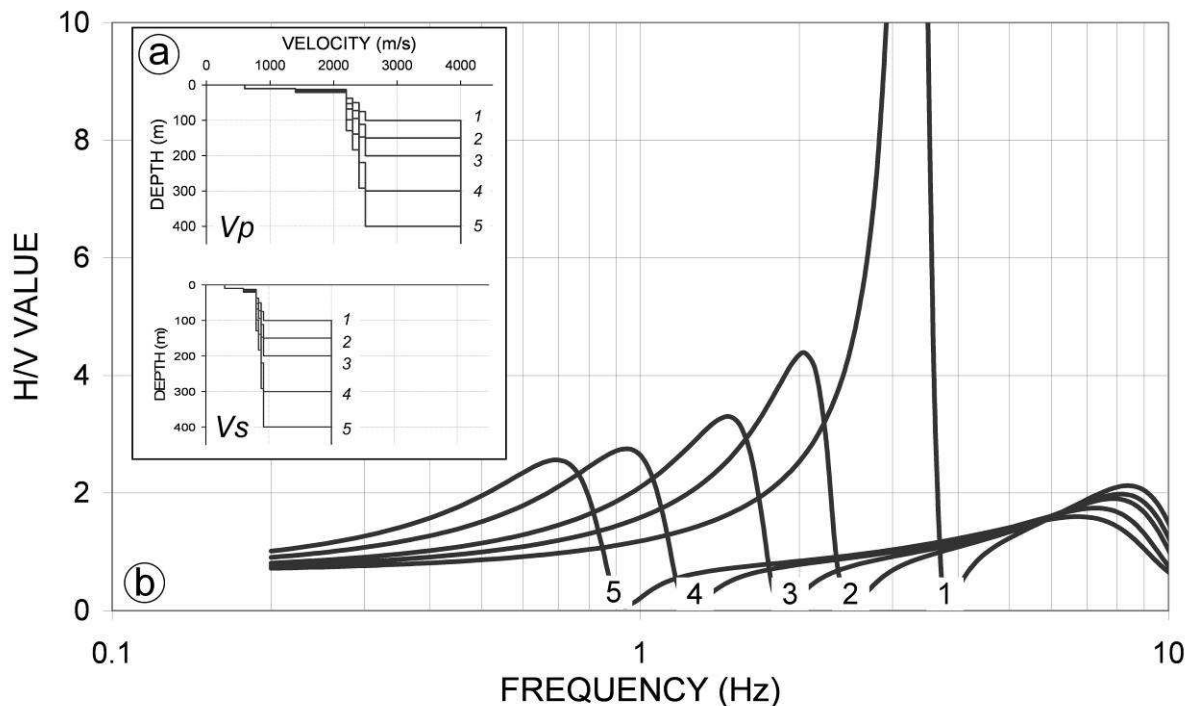
Fig. 5-9: (a) Velocity profiles for five models with different sediment thickness ( H ). (b) Computed H/V curves for different sediment thickness ( H ). 1: H=100\text{m} ; 2: H=150\text{m} ; 3: H=200\text{m} ; 4: H=300\text{m} ; 5: H=400\text{m} .
