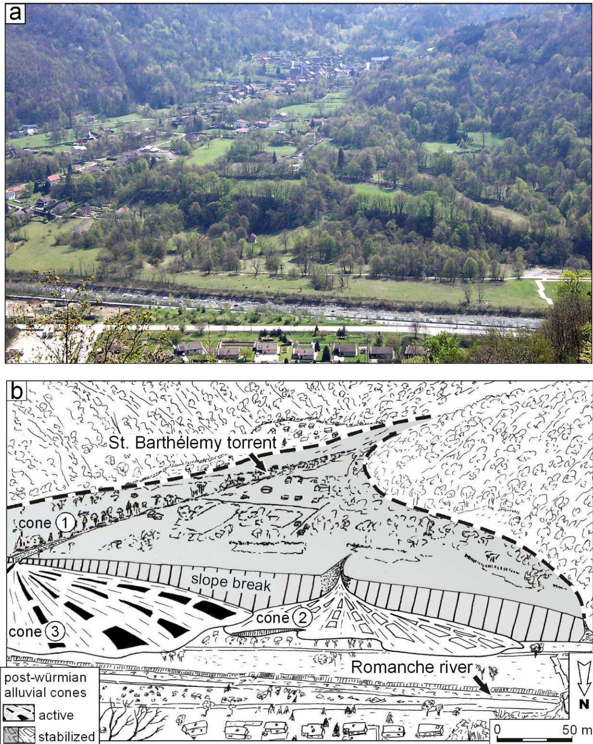
Fig. 5-4: (a) Southward view of the Saint Barthélemy post-würmian alluvial system seen from north. The area photographed is located on Fig. 5-2a. (b) Interpretation of the alluvial system as three nested cones. The stabilized cone 1 displays a rectilinear slope break.
