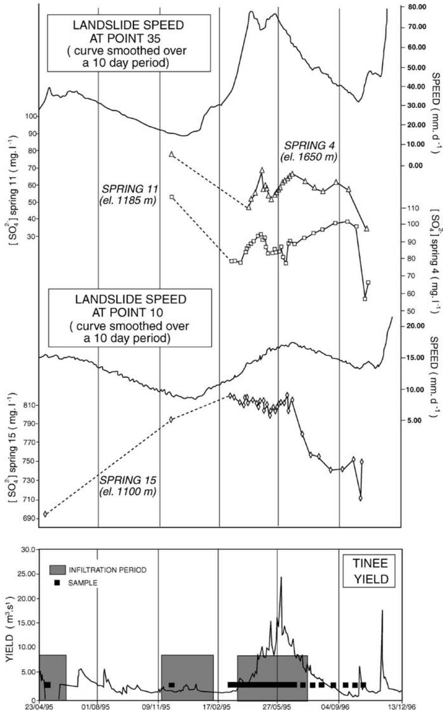
Fig. 6. Comparison between \text{SO}_4^{2-} content of spring waters and speed variations for two representative points of the moving zone at the La Clapière site
